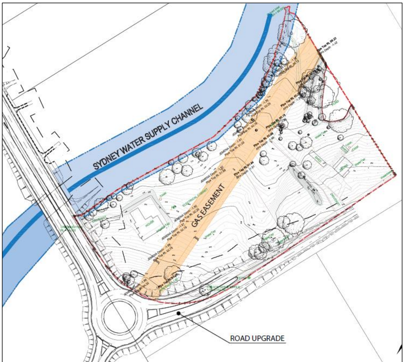
Figure 2: Site Survey Plan
